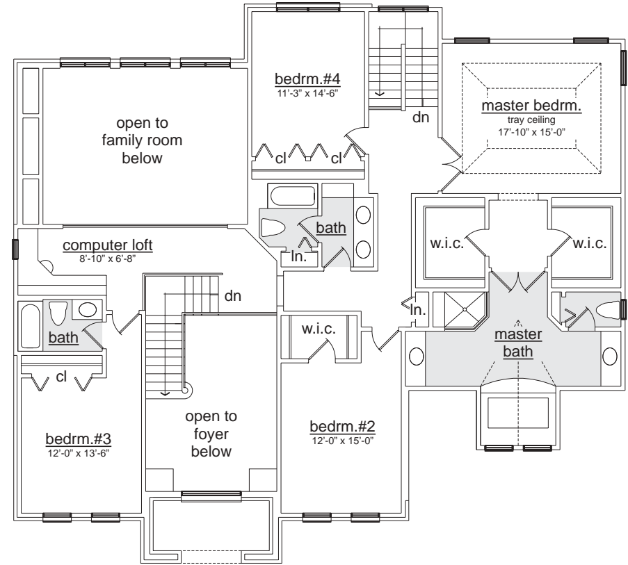
SECOND FLOOR
